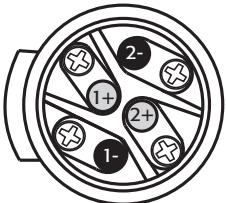
Male NL4 Wiring – Figura 3 –
