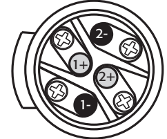
Male NL4 Wiring – Figure 3 –
