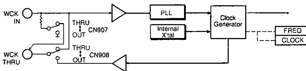
Wordclock Block Diagram
