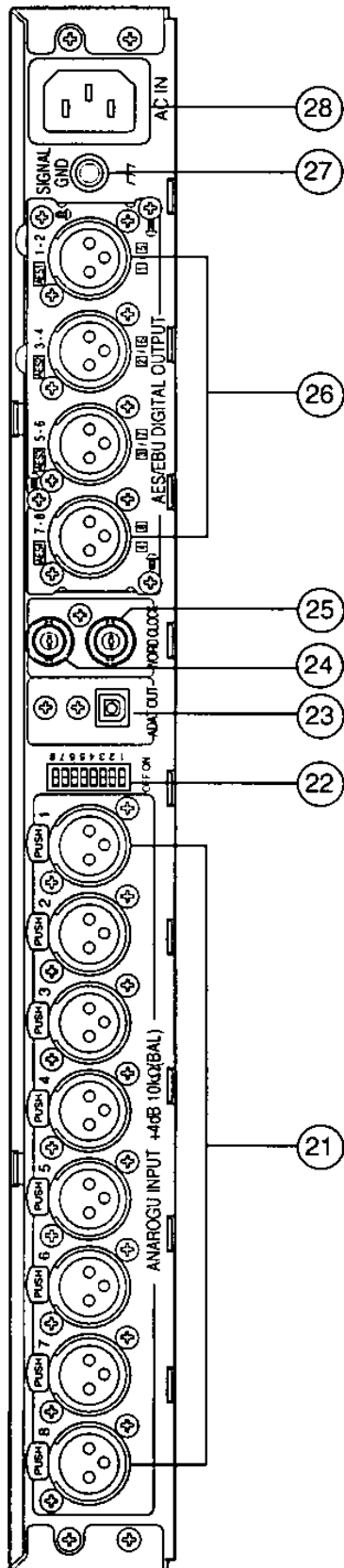
WZ-AD96 Rear Panel
