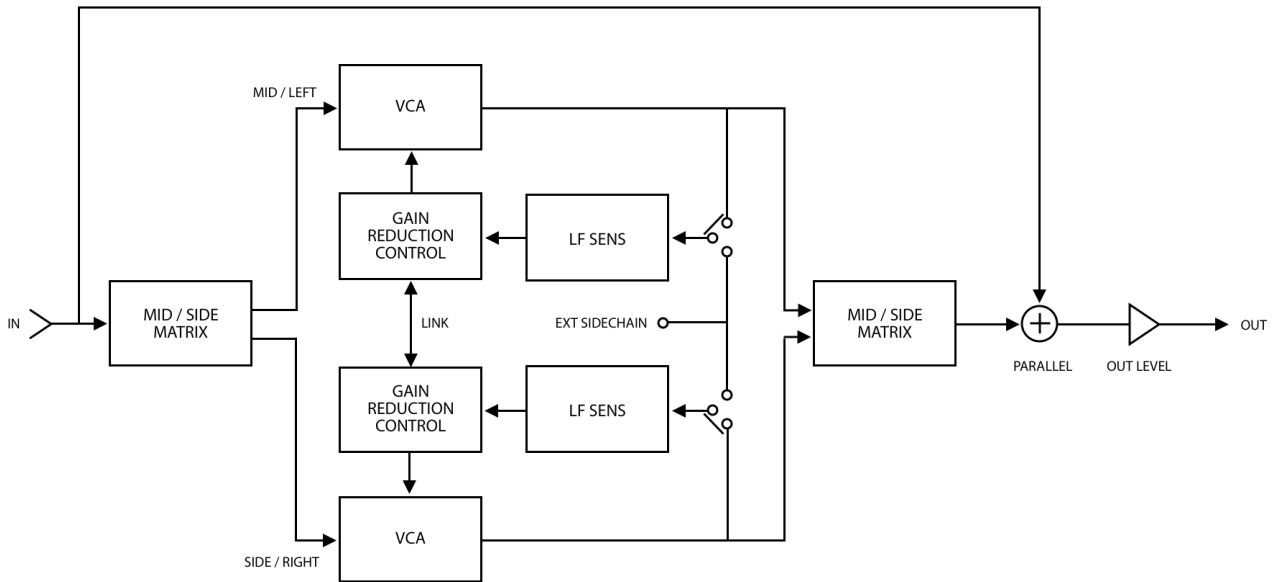
This diagram describes the COMP76 internal sections and the way they are interconnected.
